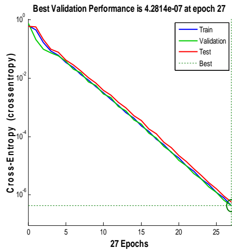
Figure 6. Training Performance
