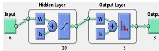
Figure.2. Network Architecture
