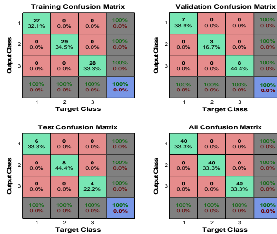
Figure.7 Confusion Matrix
